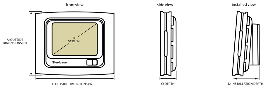
RoomWizard Room Scheduling System (RW 10) Dimensions
